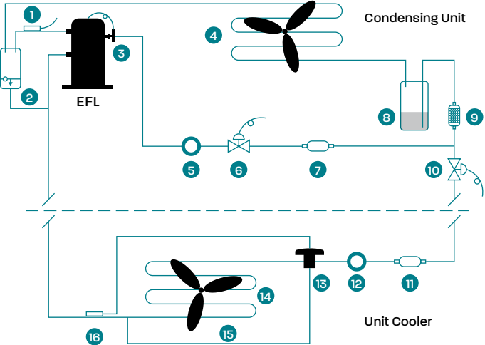
Liquid injection schematic
