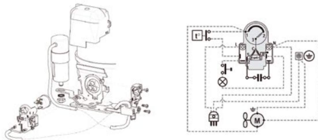
SM02 - EMT/NE SERIES RSCR TSD European Version
