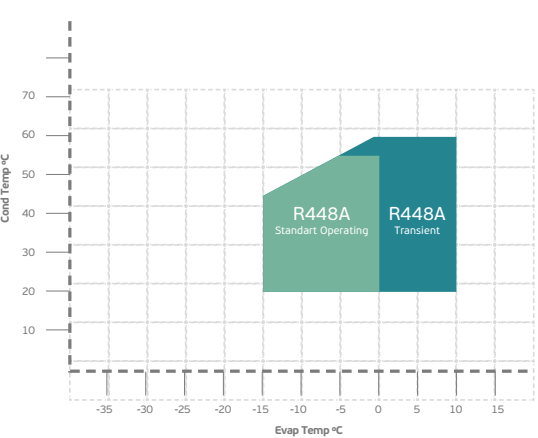
MBP (R448A) - Standard Operating Envelope
