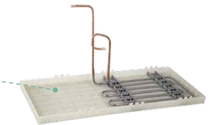
Support holding the hot-loop in position after installation and transportation to assure performance
