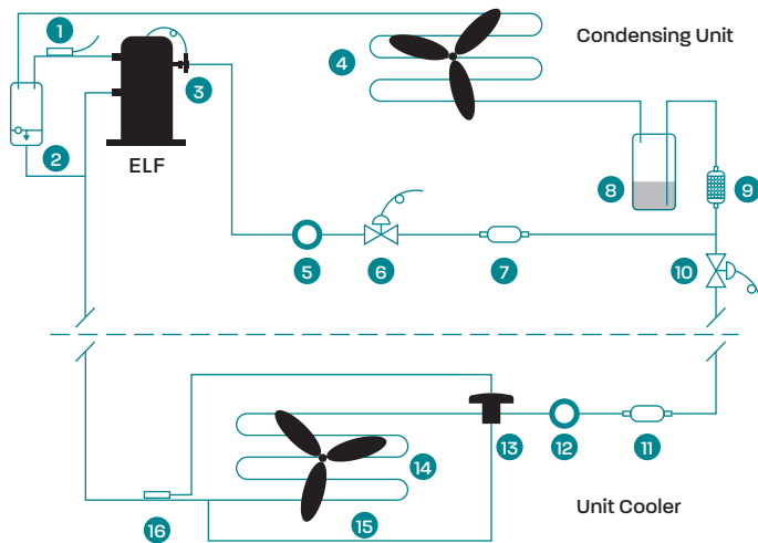
Liquid Injection without DTC schematic
