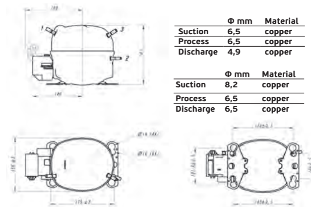
DWG10 - EM SERIES Universal Base Plate
