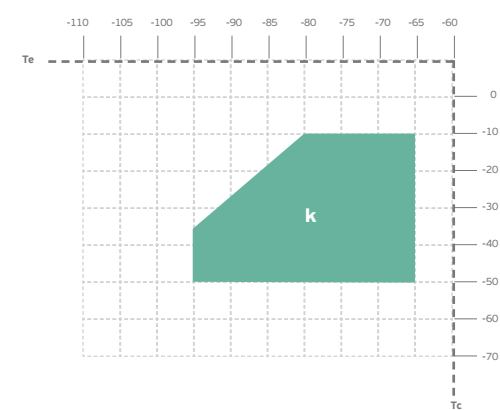
ULBP R508B/R170 - second stage of cascade
