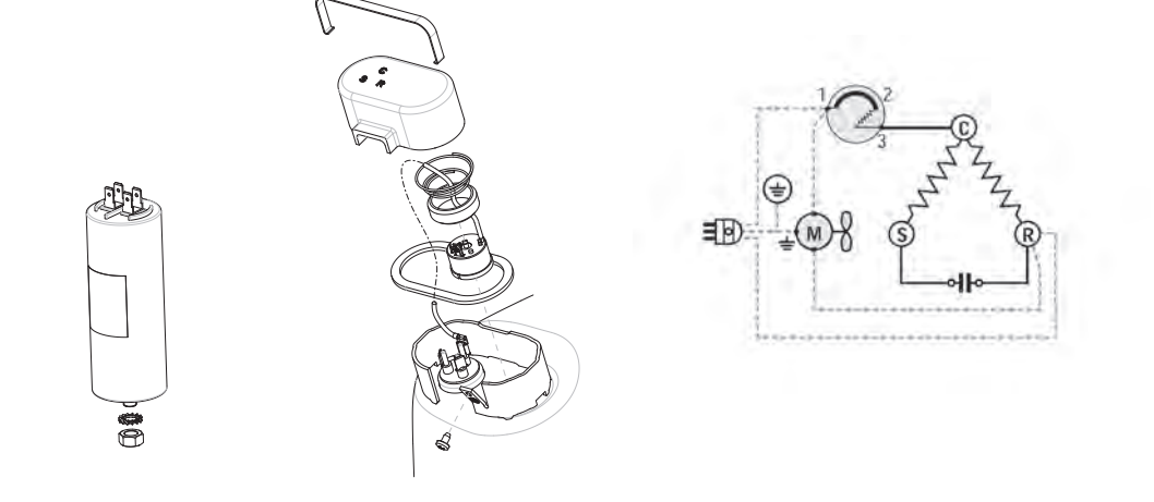
SM16 - NJ SERIES CSR Box (Internal Overload Protector)
