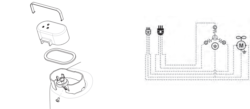
SM19 - NT SERIES CSIR Terminal Board
