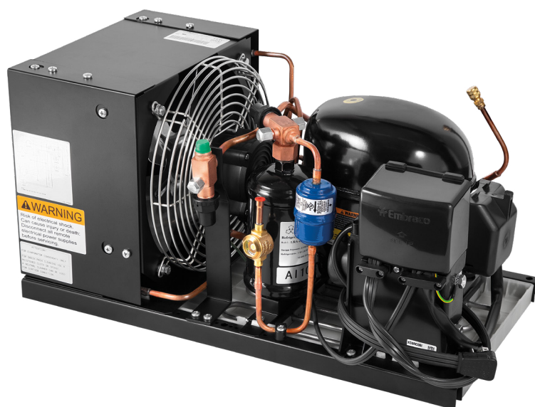
Condensing Unit with Evaporative Drain Pan
