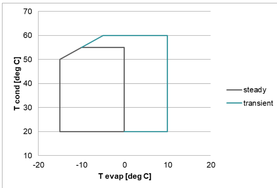
Fig.3 - Restricted R448A/R449A MBP Envelope (max. return 20°C)
