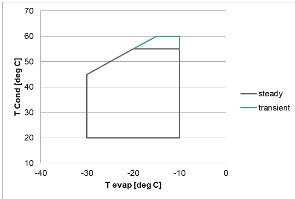
Fig.4 - Restricted R448A/R449A LBP Envelope (max. superheat 10K)
